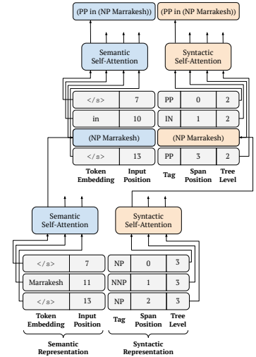
Figure 3: Detailed example of recursive tree aggregation.
